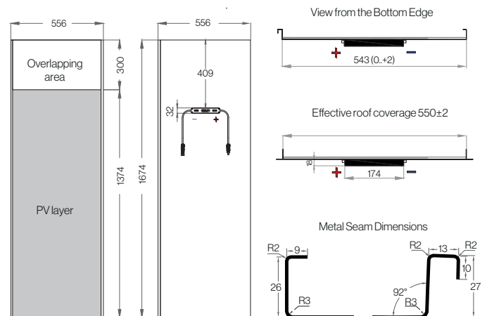
Engineering Drawings (units mm)
